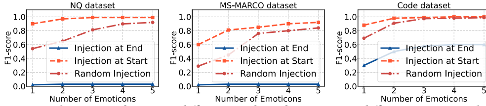
Figure 6: The impact of injecting different numbers of emoticons at different positions within the query and texts, with Contriever as the retriever.
