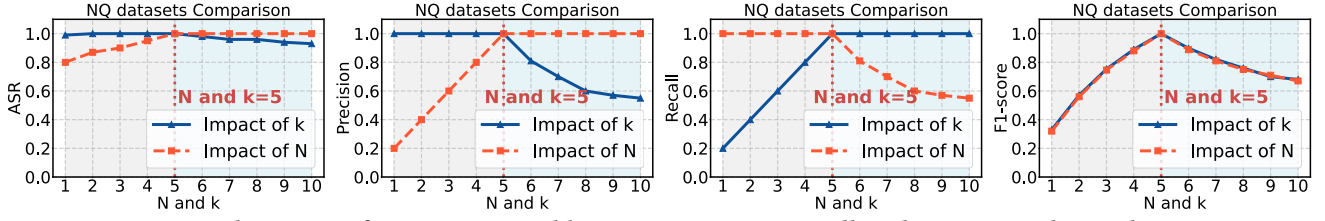
Figure 3: The impact of increasing N and k on ASR, Precision, Recall, and F1-Score in the NQ dataset.
