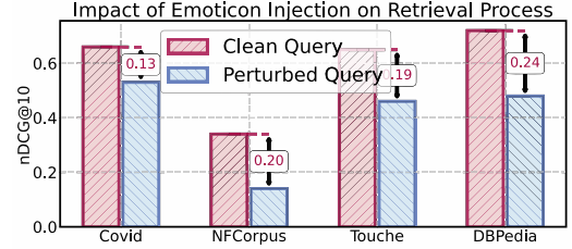
Figure 10: Emoticon Perturbation lowers retrieval performance on the BEIR benchmark
