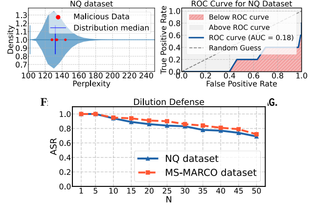
Figure 13: Dilution Defense against EmoRAG
